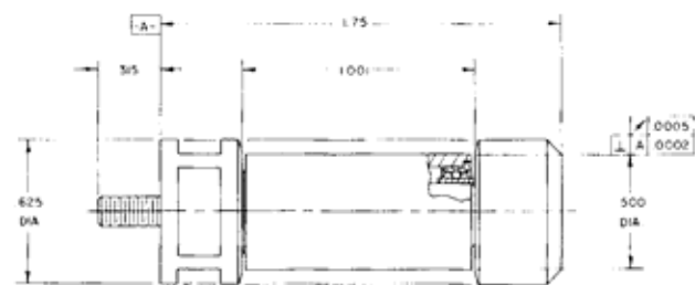
Figure 36-3—Naval audio recording system, stationary-flange tape guide.
