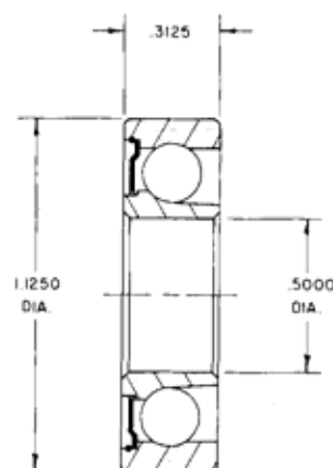
Figure 35-5, 35-6 —These bearings are used in actuator motors which are driven by bleed air from gas turbine engines. Temperatures are typically 500^{\circ} C coupled with high speed rotation.
