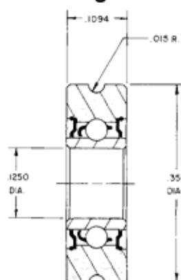
Figure 34-7 —Wire guide bearing with a full radius groove integral with the M50 tool steel outer ring. S418CHH chassis.
