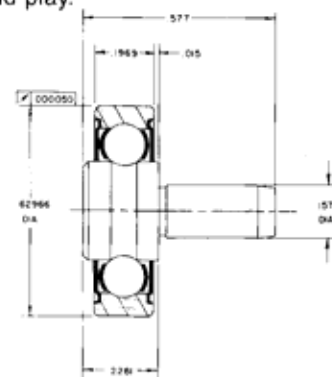
Figure 34-6 —Integral pin design, S34RHH chassis with close radial runout control.
